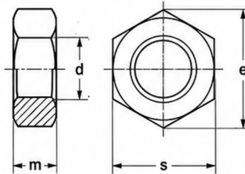
DIN 934 HEX NUTS DIMENSION TABLE (All dimensions in mm)
